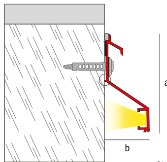
Novovierteaguas SP System with LED (optional)
